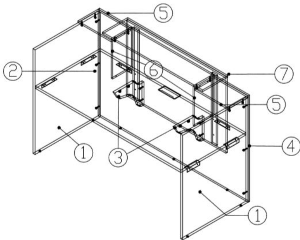
QT-M603 Assembly Drawing
