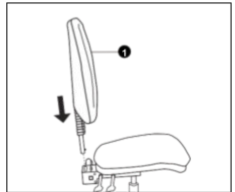
Step 3 Slide back into seat and tighten in place
