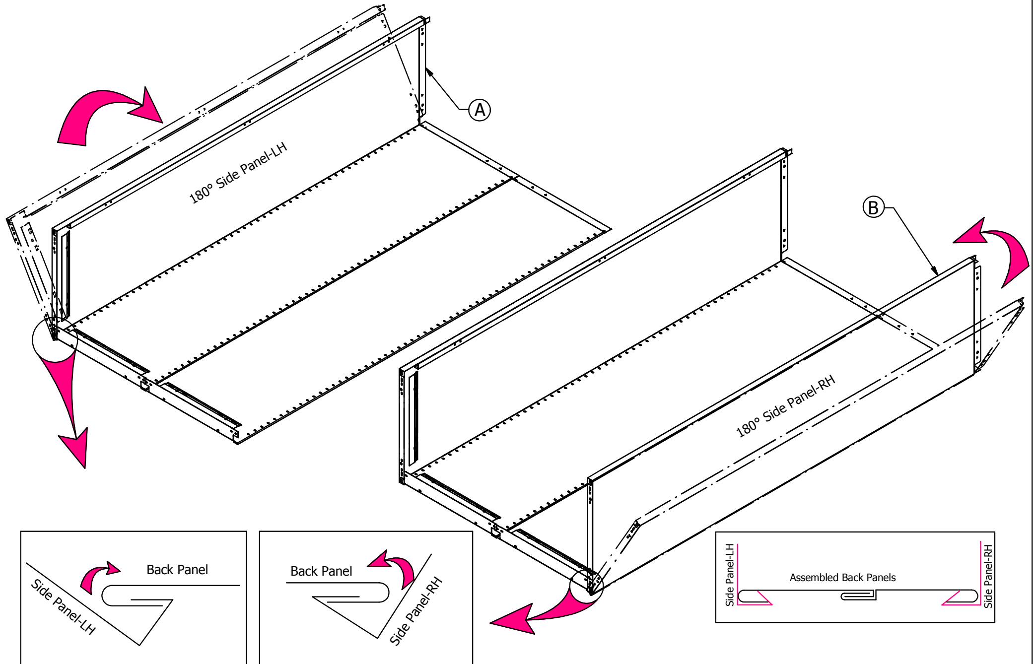
Assembly of Back & Side Panels
