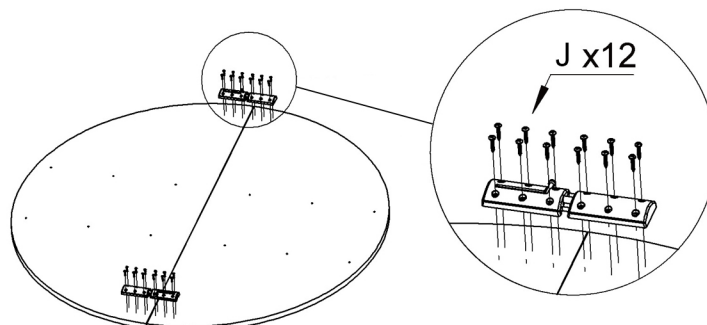
6. Put the 2 table tops (object B) together tightly and make sure they are flat. Setup the locks in the middle of the table and close to the edge as * Picture P1 shown. Keep the locks remain closed.
