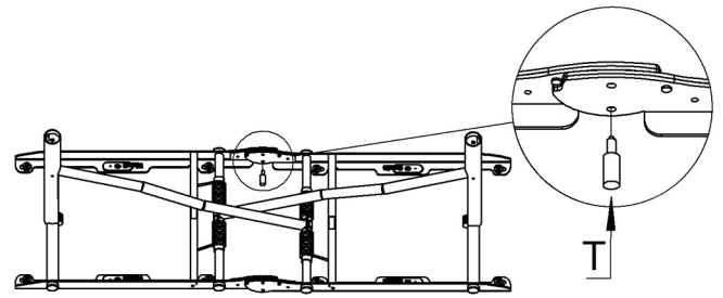
2. Insert the block pin (object T) in order to keep the frame open during the assembly.
