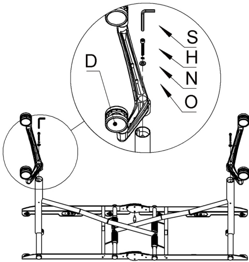
3. Setup the wheels (object D). Then turn over the frame carefully by at least 2 persons .
