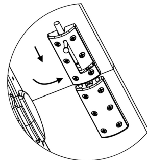
3. Lock the locks for both side
