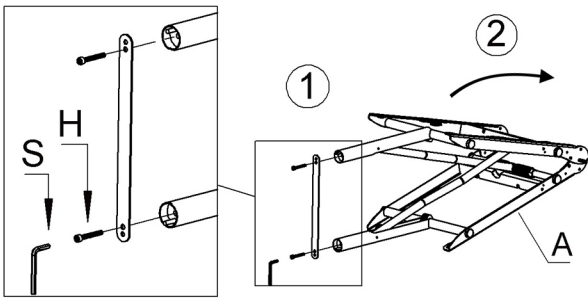
1. Open the frame (object A) carefully by releasing screws (object H).
