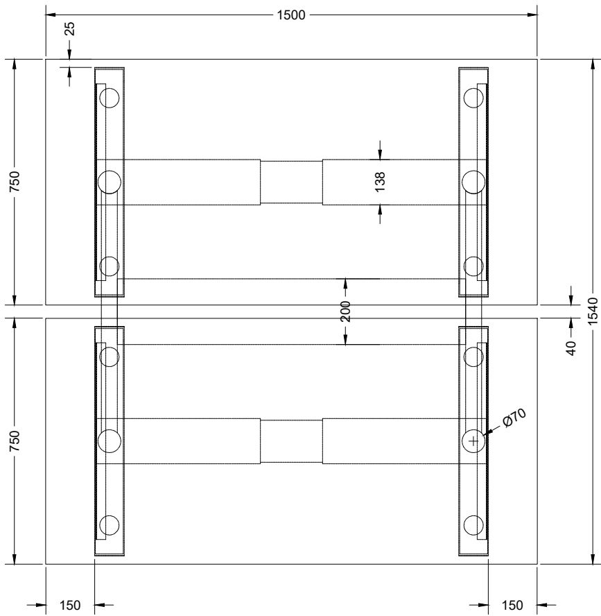
TOP VIEW
